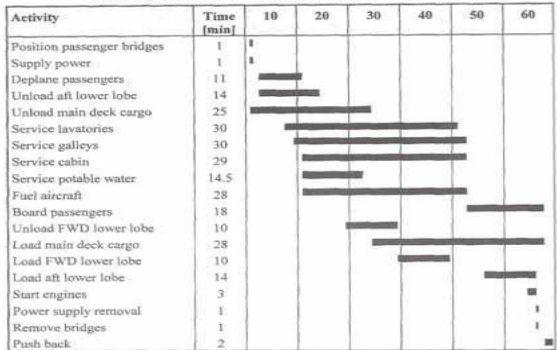
An example of the B-747 servicing at an end station turnaround
